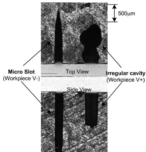
(a) Failure of micro slot machining
