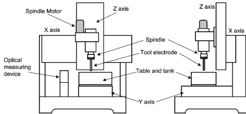
Fig. 2. Structure of desk-top miniature machine tool.
