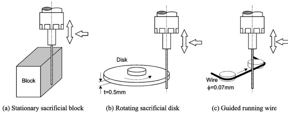
Fig. 4. Three types of sacrificial electrode for on-machine tool fabrication.
