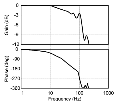
Fig. 3. Frequency characteristics of the Z-axis.
