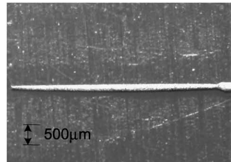
(b) Un even diameter machined using a stationary sacrificial block
