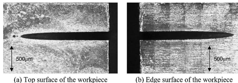
Fig. 12. Examples of the machined micro-slot.
