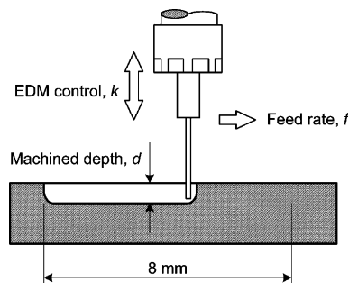
Fig. 5. Surface engraving EDM.
