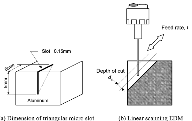
Fig. 6. Fabrication of a triangular micro-slot using linear scanning EDM.
