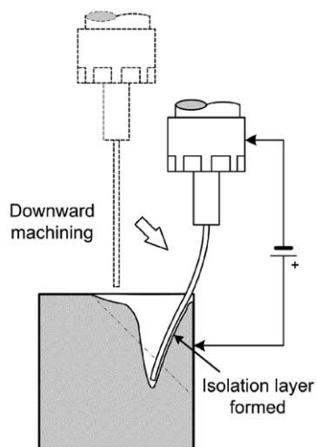
(b) Deflection of electrode in downward machining (workpiece positive)
