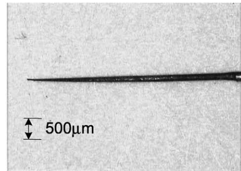
(a) Tapered tool electrode machined using a stationary sacrificial block
