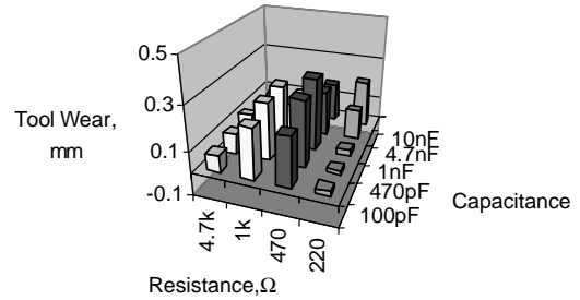
(b) EDM circuit effect on tool electrode wear
