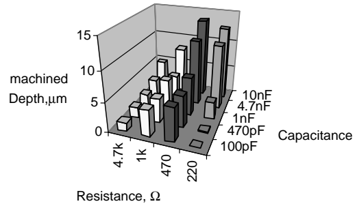
(a) EDM circuit effect on machined depth
