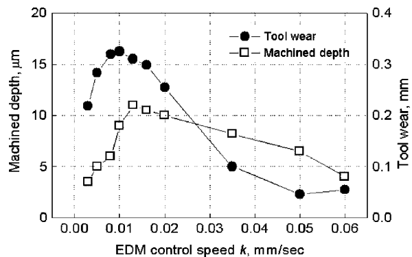
Fig. 10. Influence of EDM gap control.
