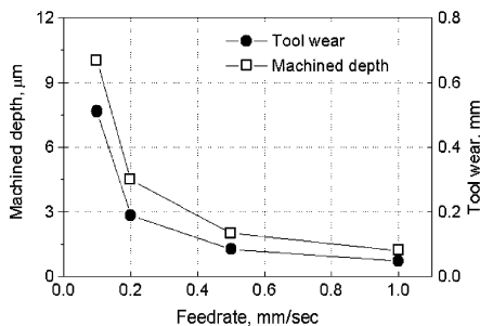
Fig. 8. Influence of feed rate on micro-EDM.
