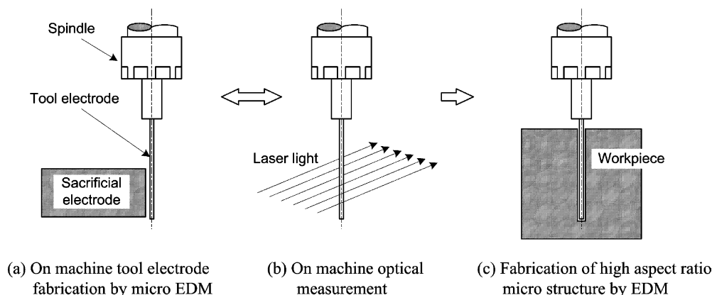
Fig. 1. Process to fabricate high-aspect ratio micro-structures using micro-EDM.
